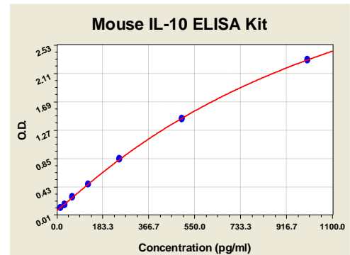
Figure 1: IL-10 Standard Curve. Using the mouse IL-10 ELISA Kit, O.D. data was graphed against IL-10 protein concentration. The TMB reaction was incubated at 37° C for 20 min.
